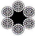
6X37 (18/12/6/1) FIBER CORE
