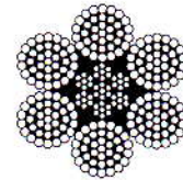
6X37 (18/12/6/1) STEEL CORE
